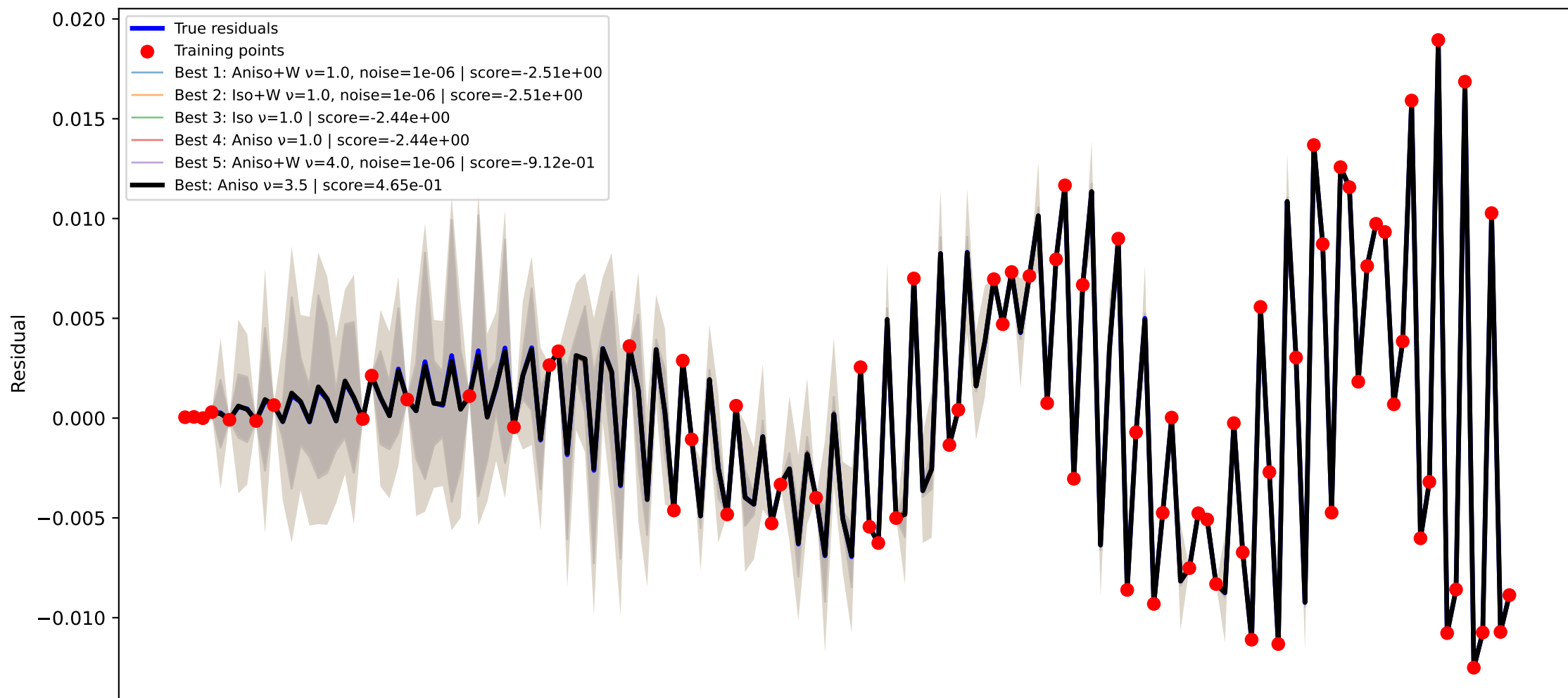
GPR kernel comparison node=38 RMSE=4.734e-05, train RMSE=1.280e-11
